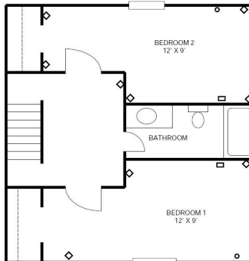
SECOND FLOOR Apt 2 (Apt 3 is a mirrored floor plan)
